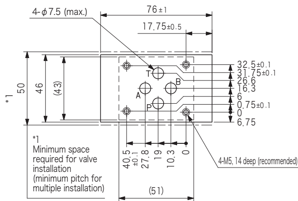
Fig. 1 Mounting dimensions
